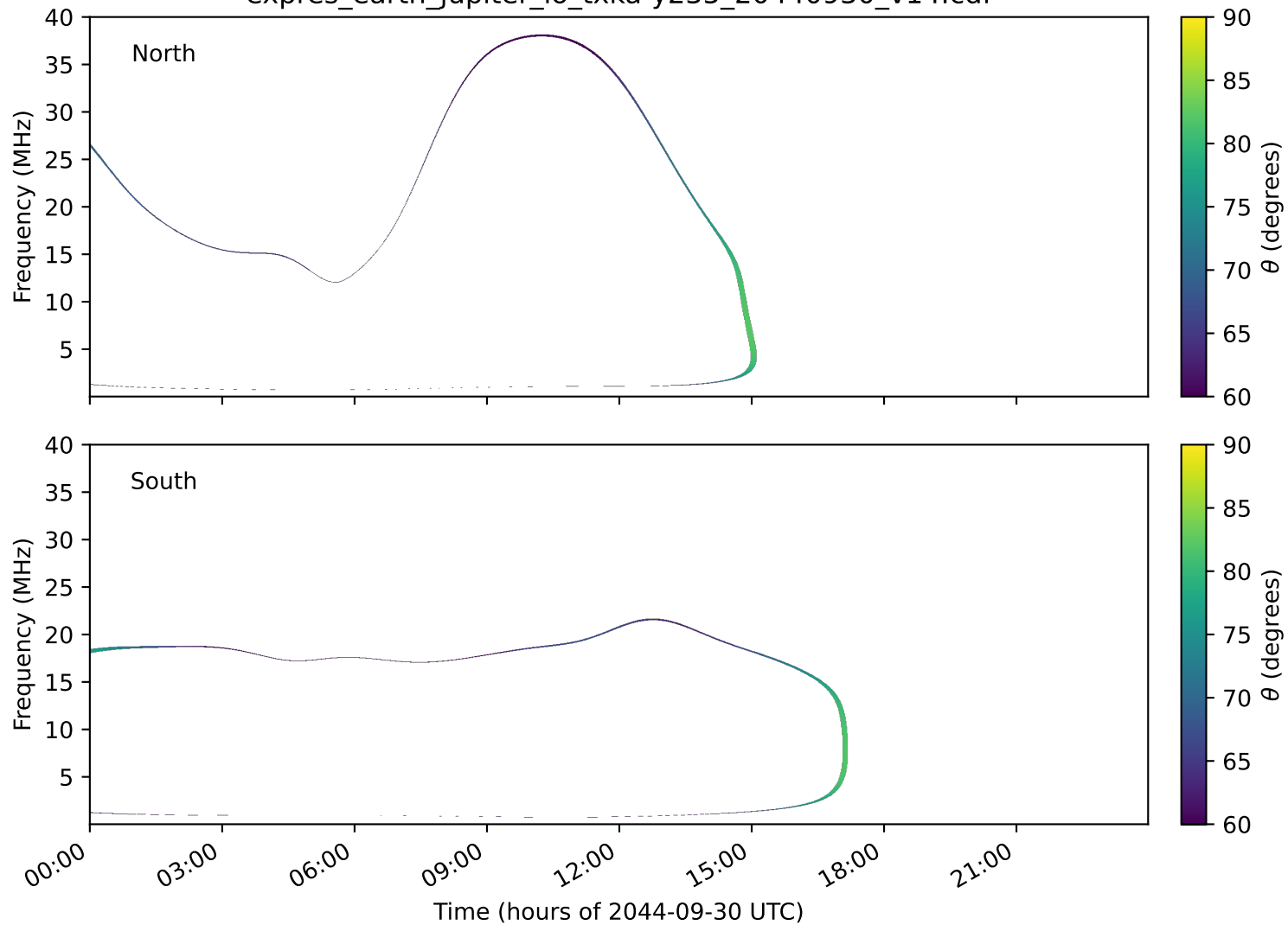
expres_earth_jupiter_io_txka-y235_20440930_v14.cdf
