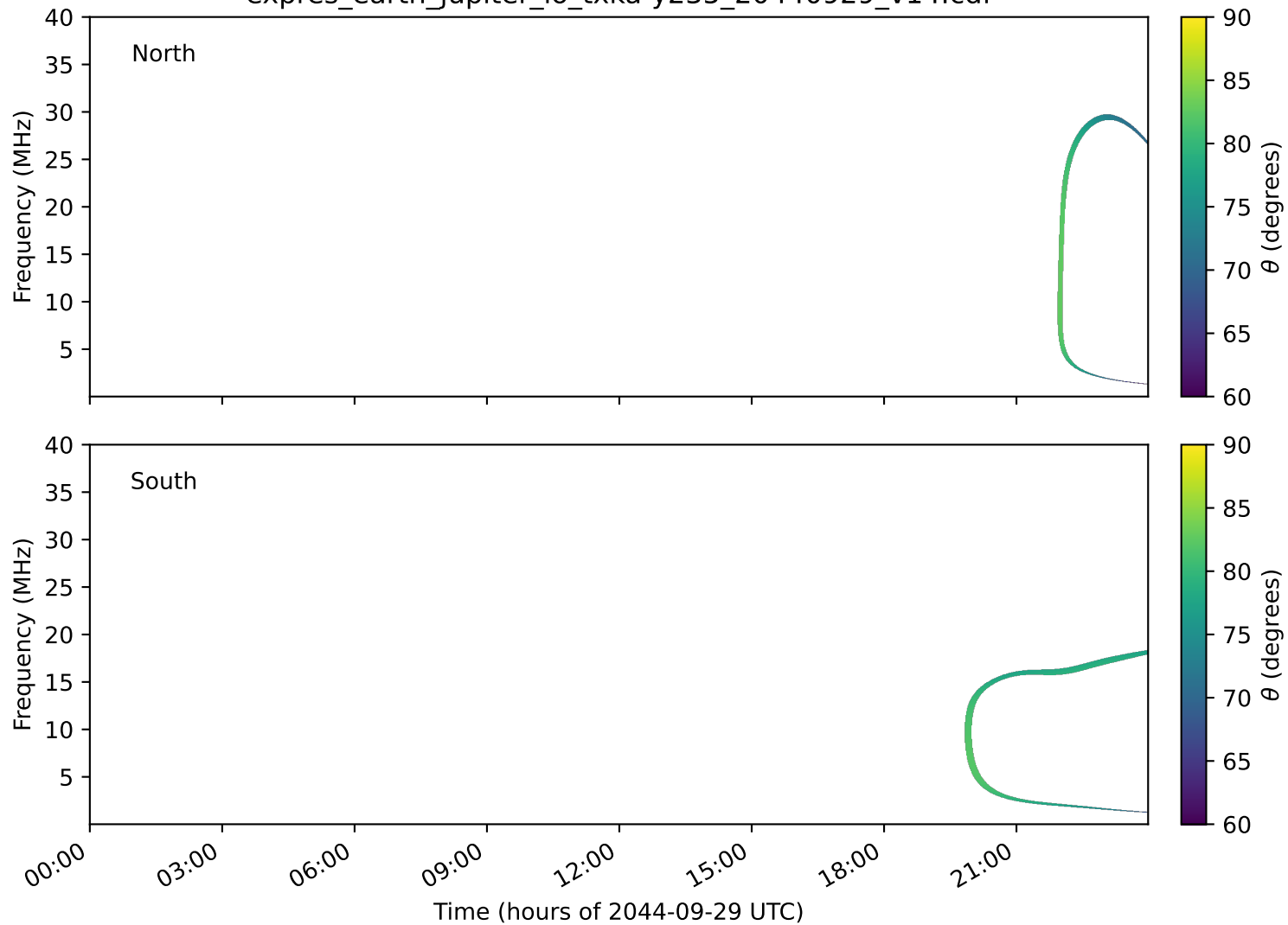
expres_earth_jupiter_io_txka-y235_20440929_v14.cdf
