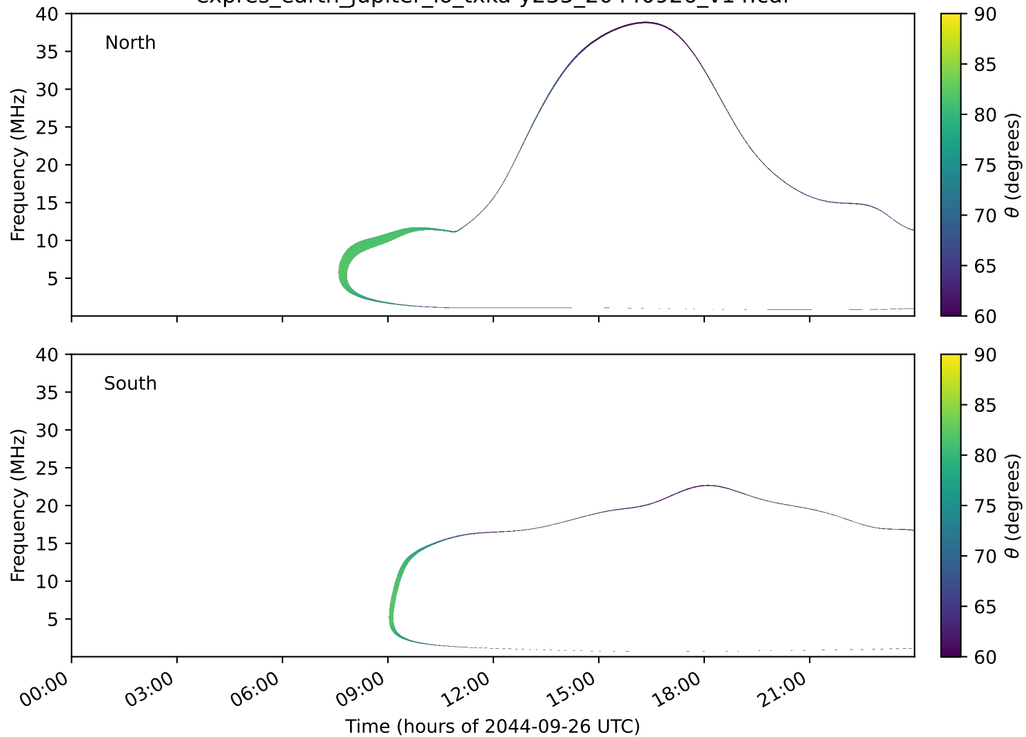
expres_earth_jupiter_io_txka-y235_20440926_v14.cdf
