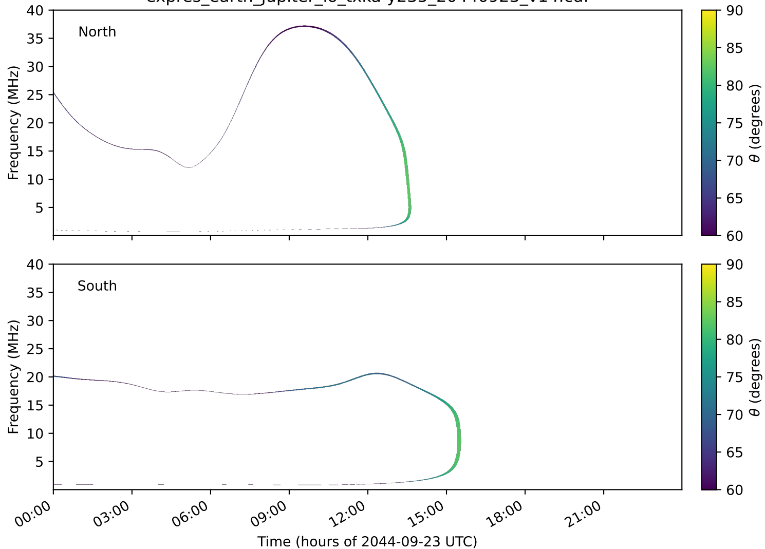
expres_earth_jupiter_io_txka-y235_20440923_v14.cdf
