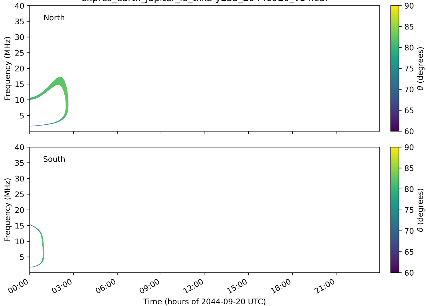
expres_earth_jupiter_io_txka-y235_20440920_v14.cdf
