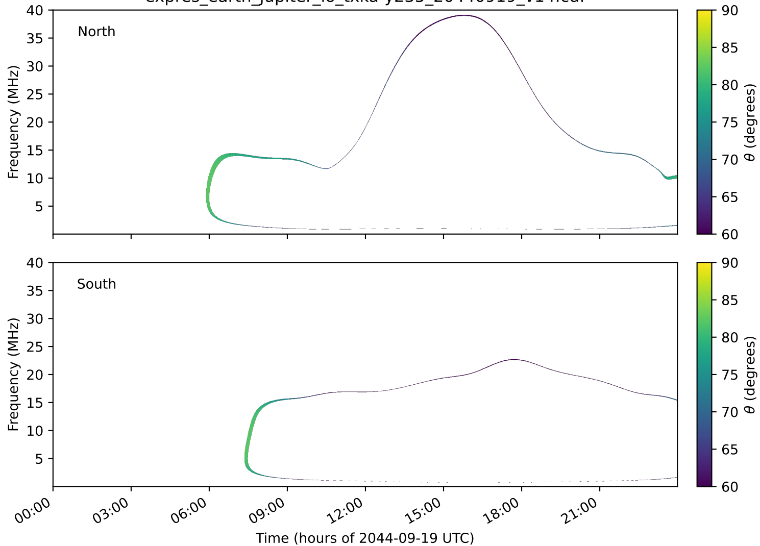
expres_earth_jupiter_io_txka-y235_20440919_v14.cdf
