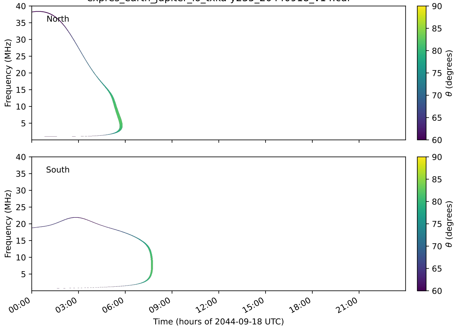
expres_earth_jupiter_io_txka-y235_20440918_v14.cdf
