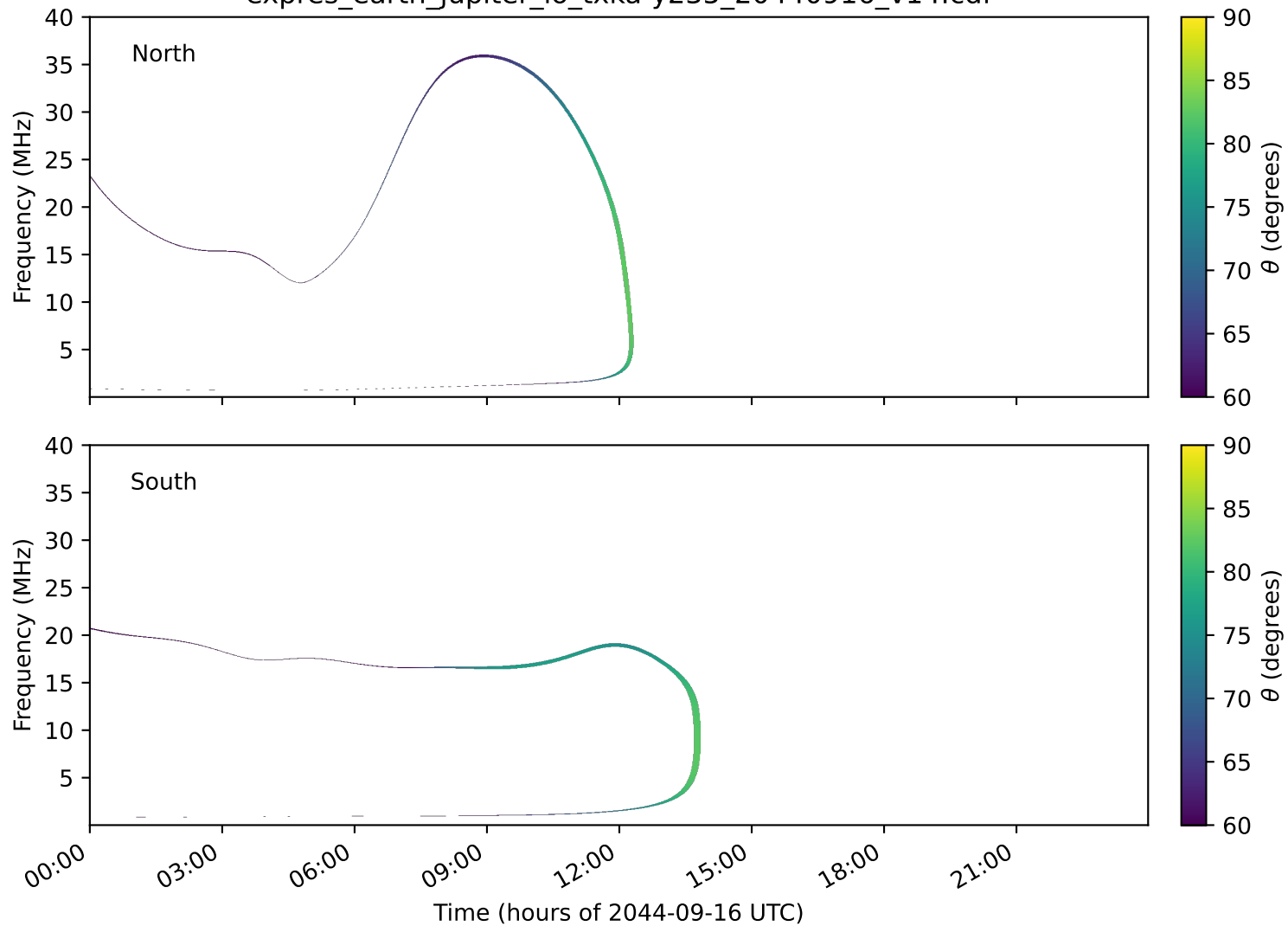
expres_earth_jupiter_io_txka-y235_20440916_v14.cdf
