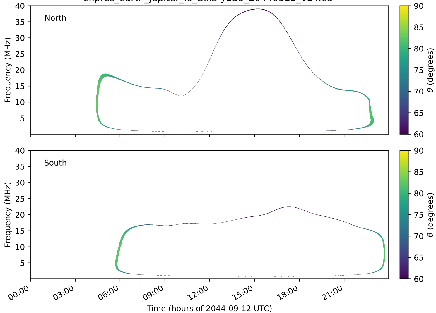
expres_earth_jupiter_io_txka-y235_20440912_v14.cdf
