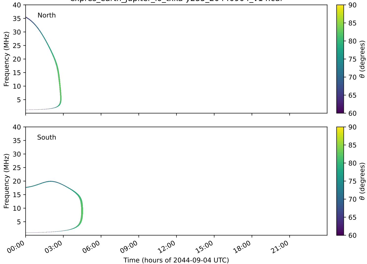
expres_earth_jupiter_io_txka-y235_20440904_v14.cdf
