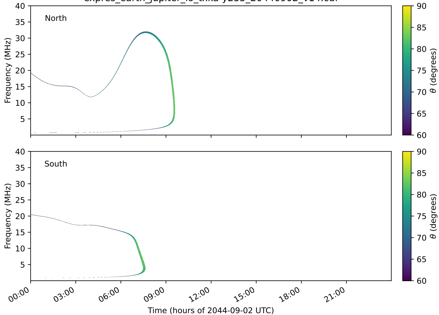
expres_earth_jupiter_io_txka-y235_20440902_v14.cdf
