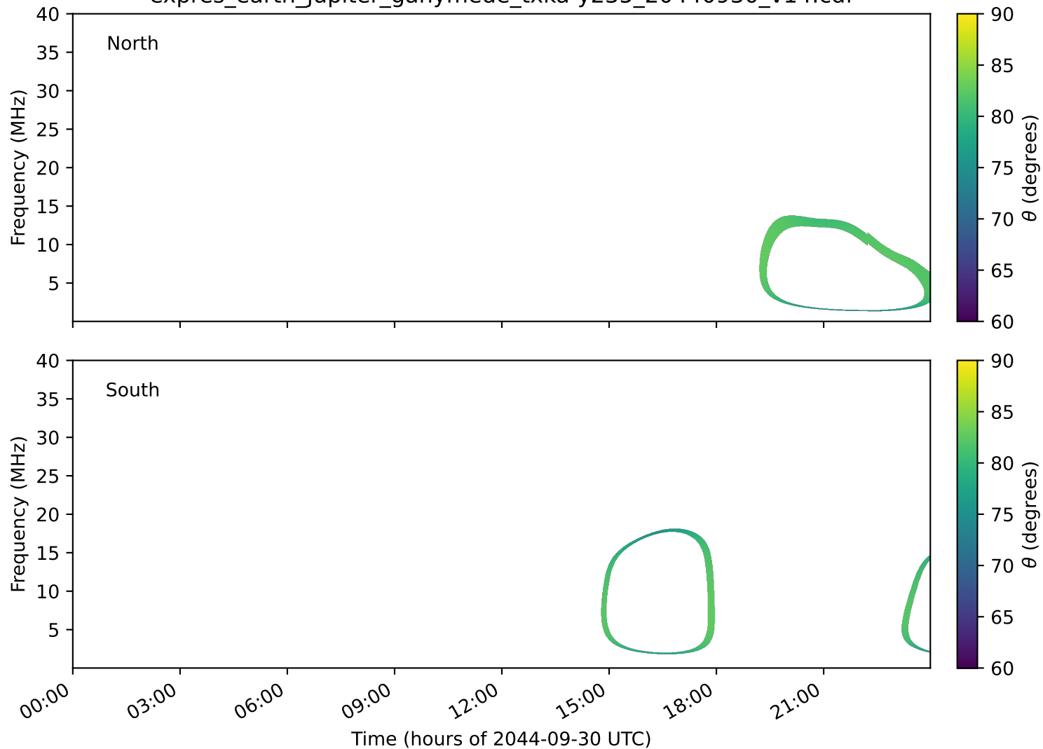
expres_earth_jupiter_ganymede_txka-y235_20440930_v14.cdf
