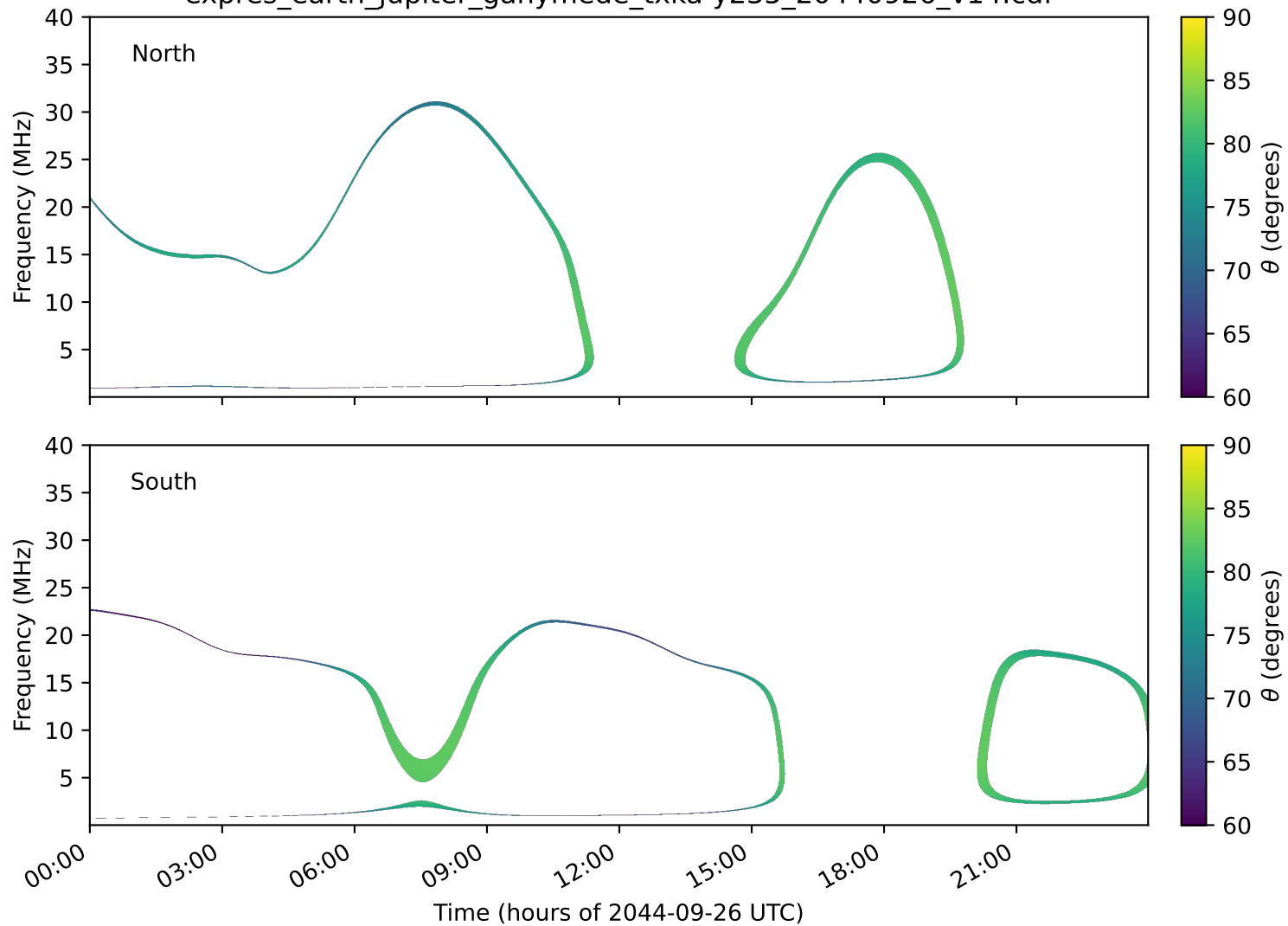
expres_earth_jupiter_ganymede_txka-y235_20440926_v14.cdf
