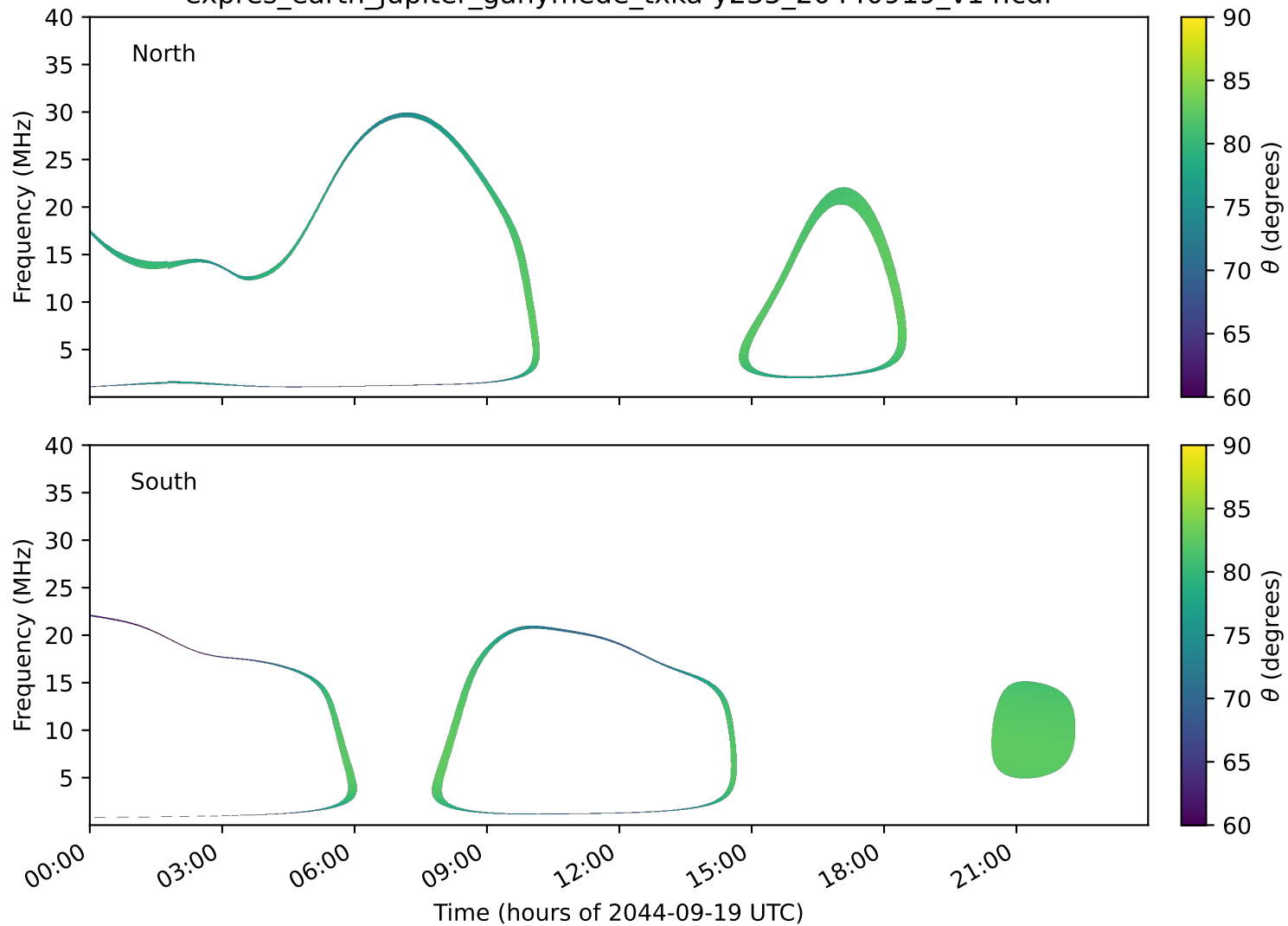
expres_earth_jupiter_ganymede_txka-y235_20440919_v14.cdf
