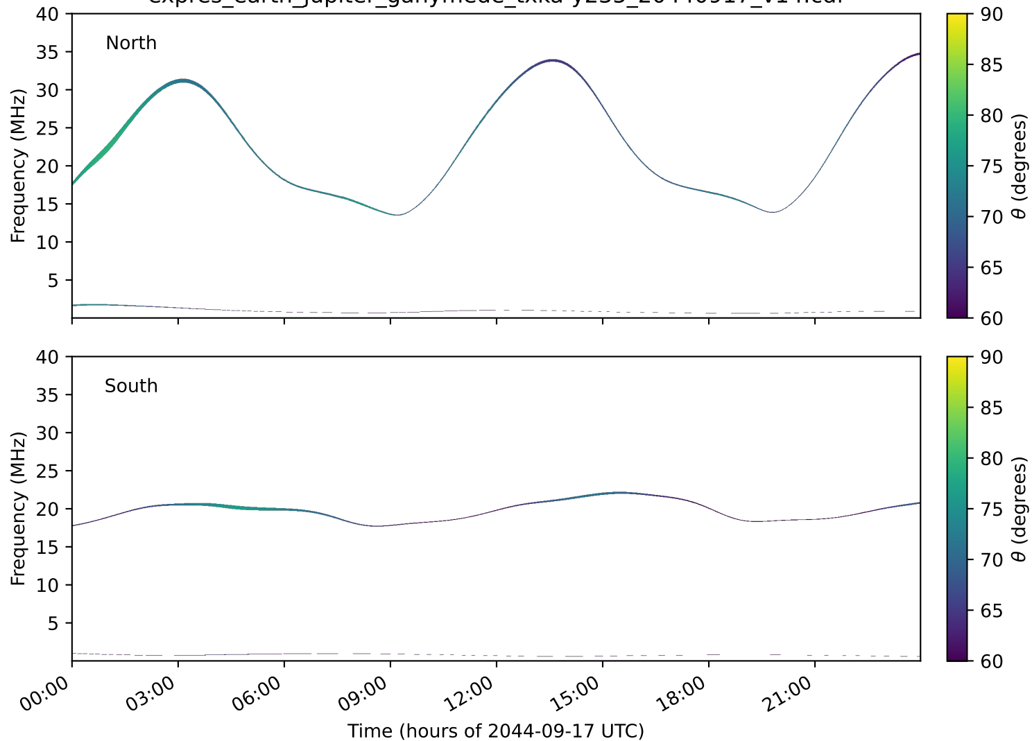
expres_earth_jupiter_ganymede_txka-y235_20440917_v14.cdf
