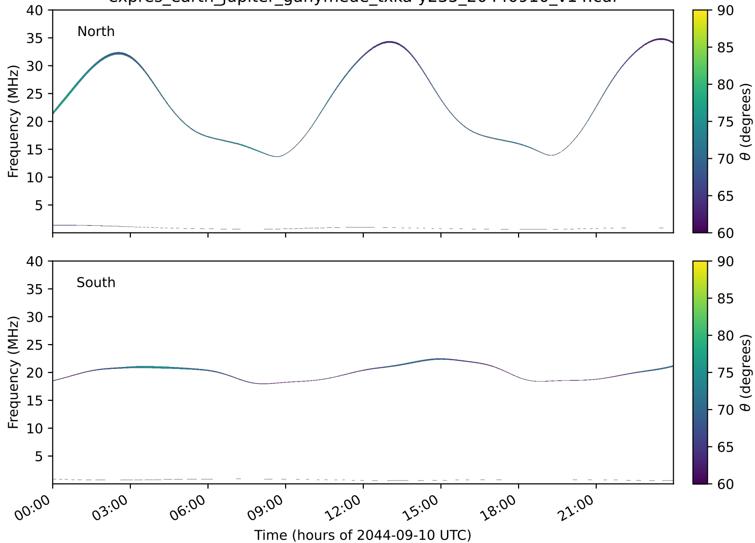
expres_earth_jupiter_ganymede_txka-y235_20440910_v14.cdf
