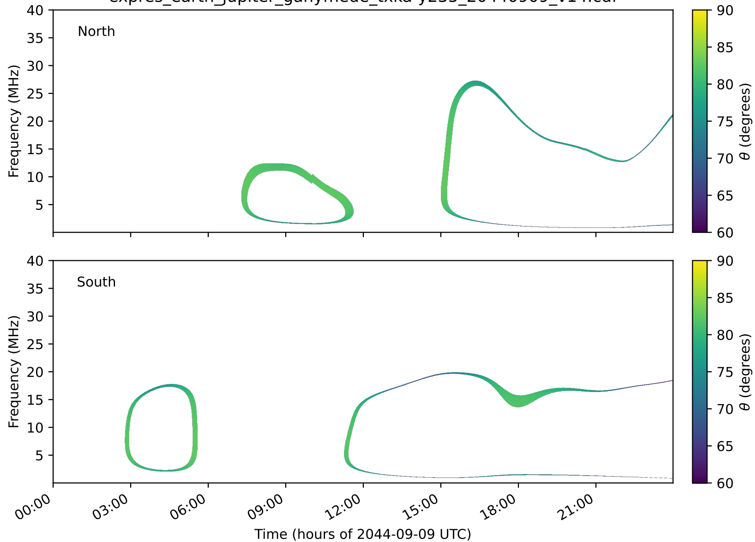
expres_earth_jupiter_ganymede_txka-y235_20440909_v14.cdf
