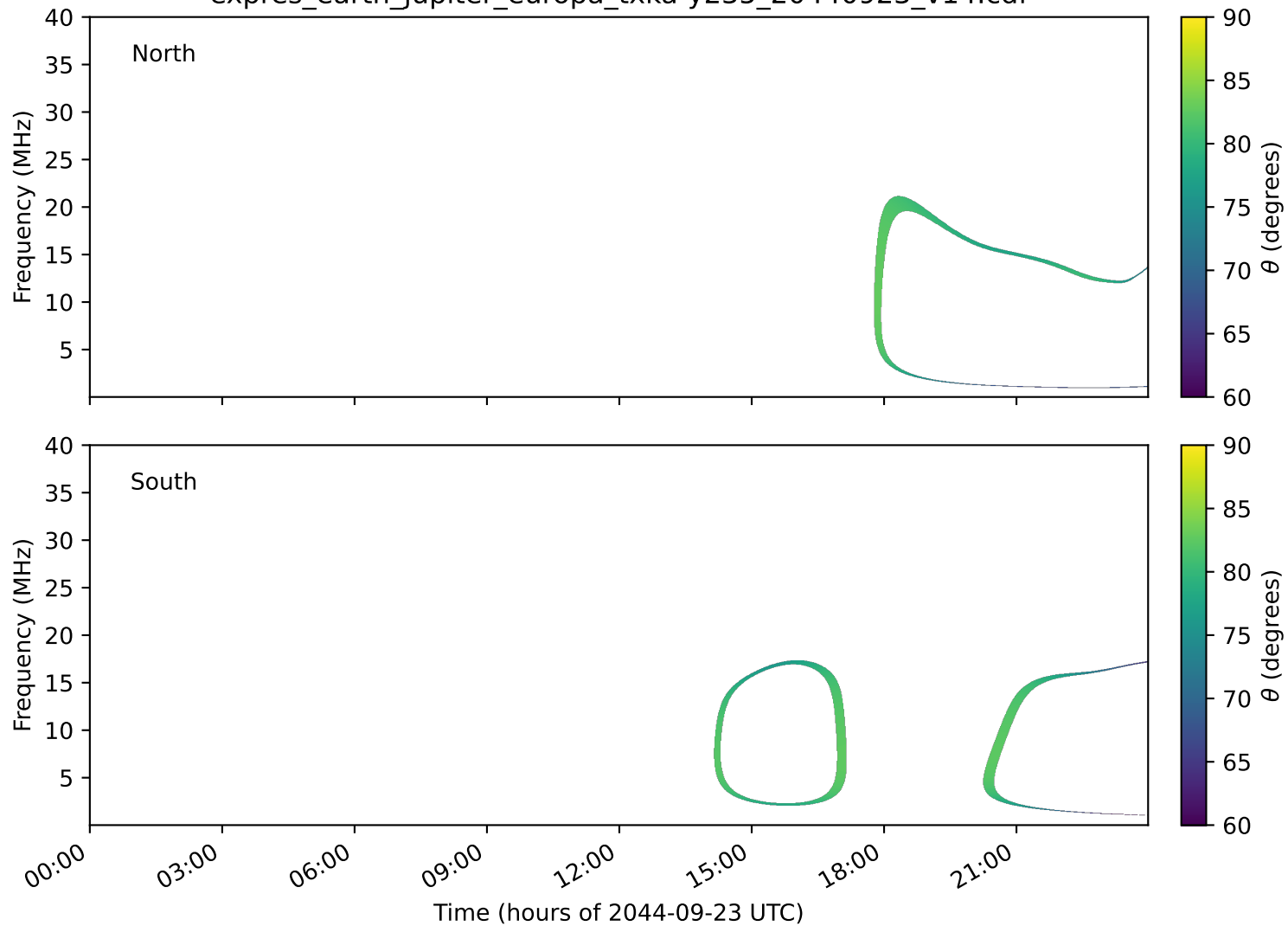
expres_earth_jupiter_europa_txka-y235_20440923_v14.cdf
