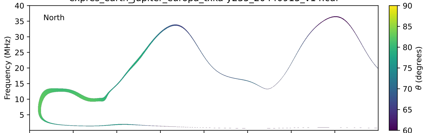
expres_earth_jupiter_europa_txka-y235_20440913_v14.cdf
