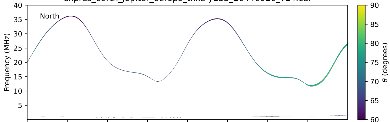
expres_earth_jupiter_europa_txka-y235_20440910_v14.cdf
