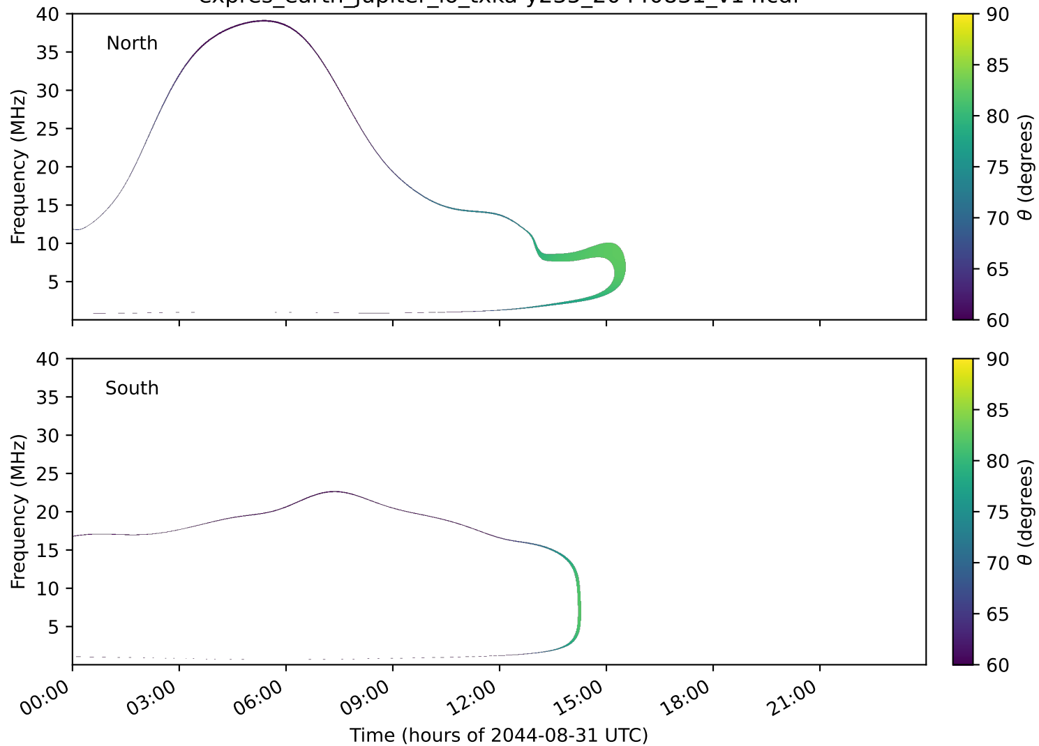
expres_earth_jupiter_io_txka-y235_20440831_v14.cdf
