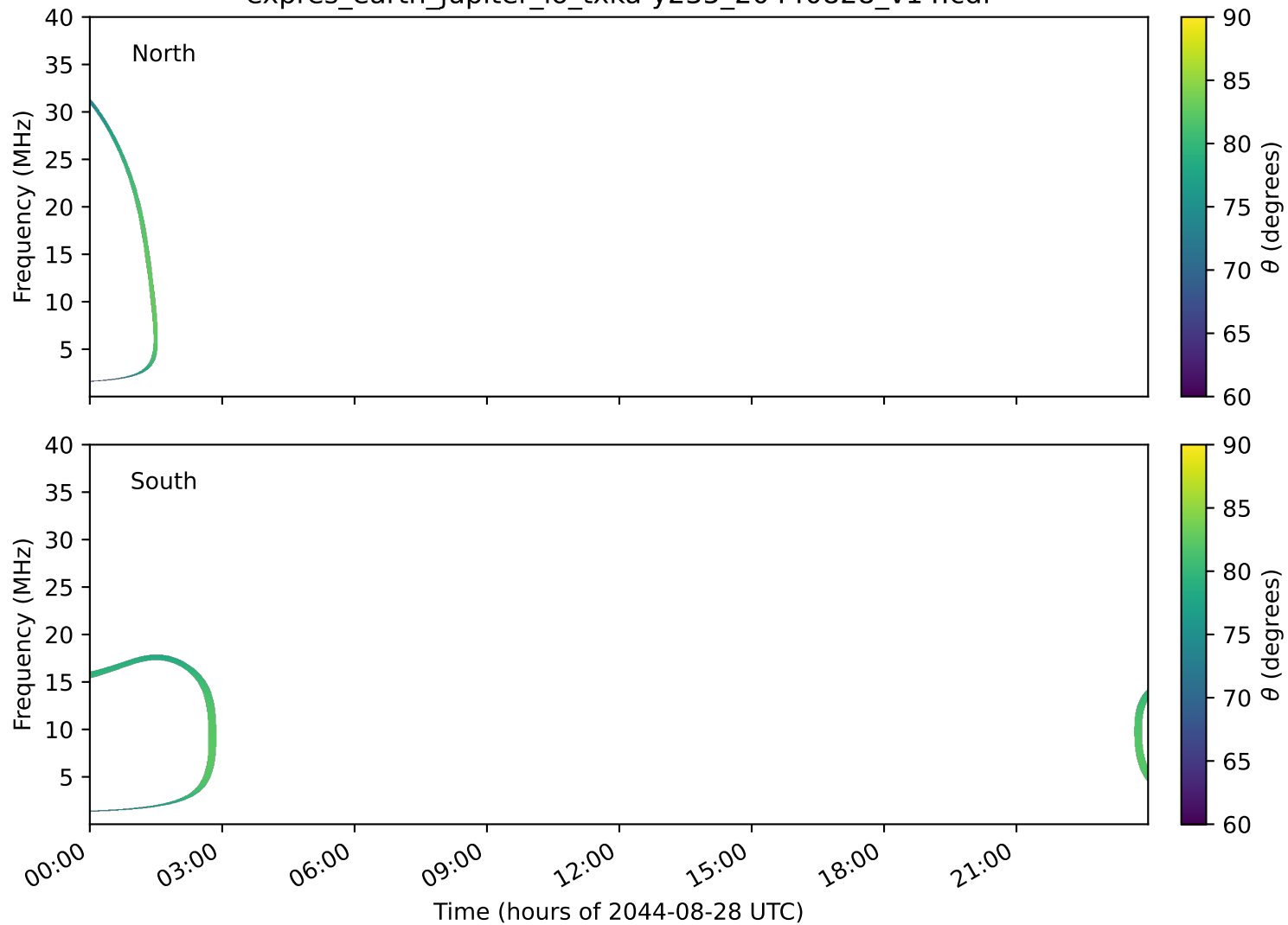
expres_earth_jupiter_io_txka-y235_20440828_v14.cdf
