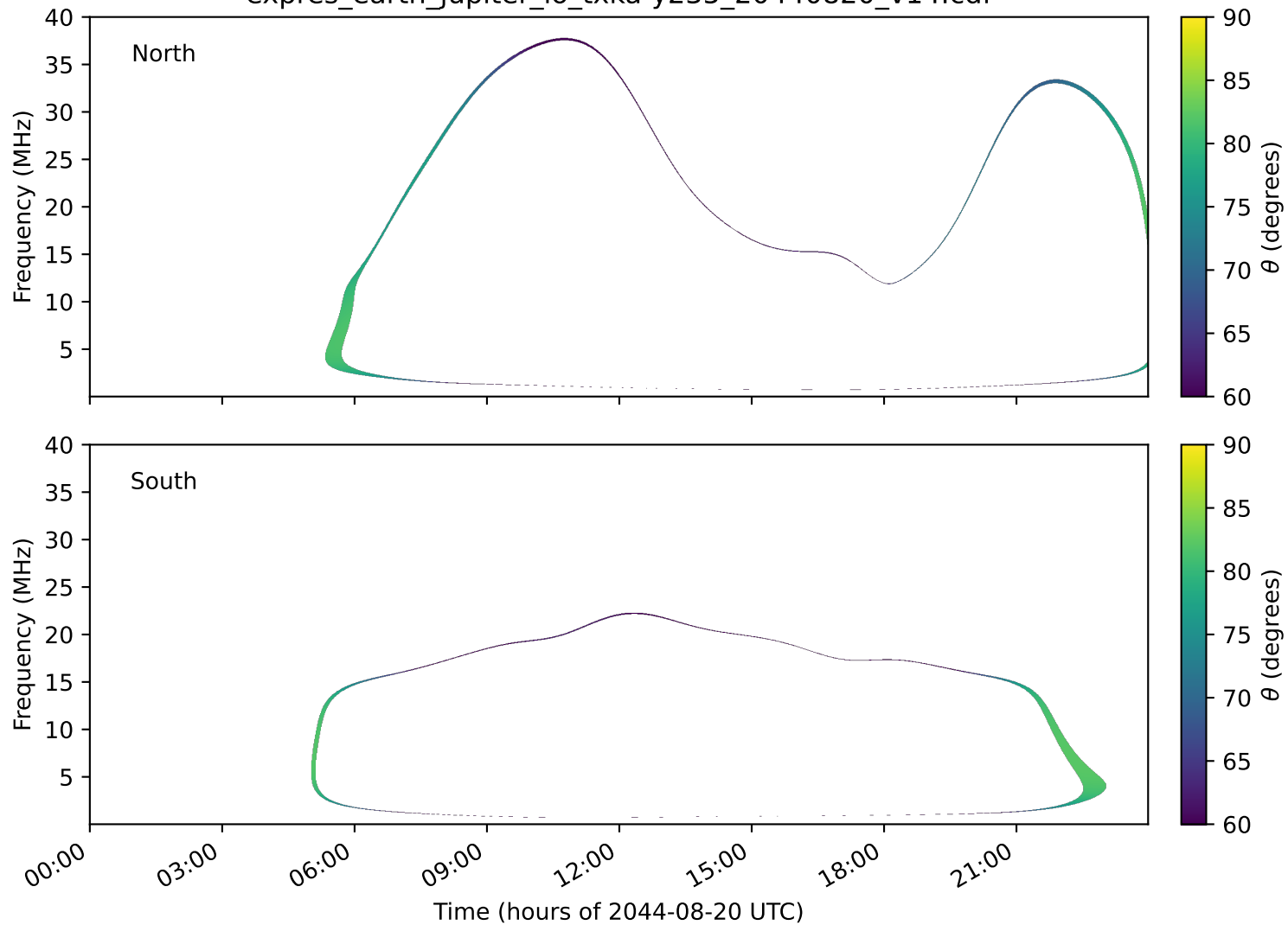
expres_earth_jupiter_io_txka-y235_20440820_v14.cdf
