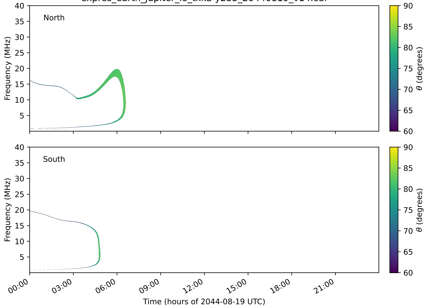
expres_earth_jupiter_io_txka-y235_20440819_v14.cdf
