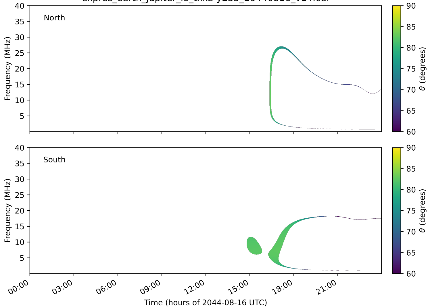
expres_earth_jupiter_io_txka-y235_20440816_v14.cdf
