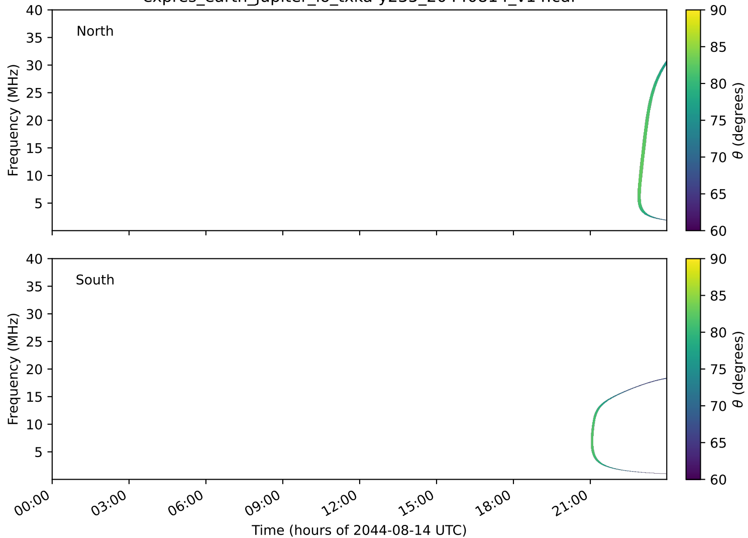
expres_earth_jupiter_io_txka-y235_20440814_v14.cdf
