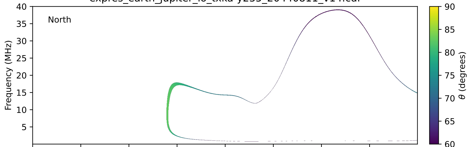
expres_earth_jupiter_io_txka-y235_20440811_v14.cdf
