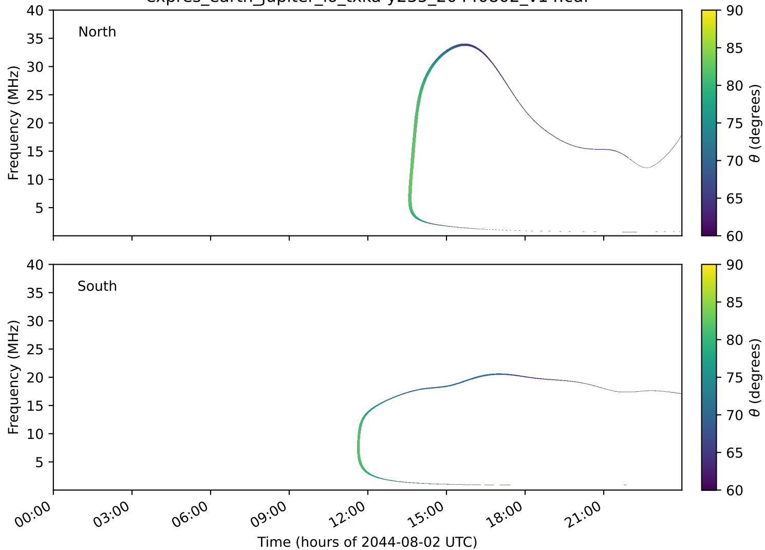
expres_earth_jupiter_io_txka-y235_20440802_v14.cdf
