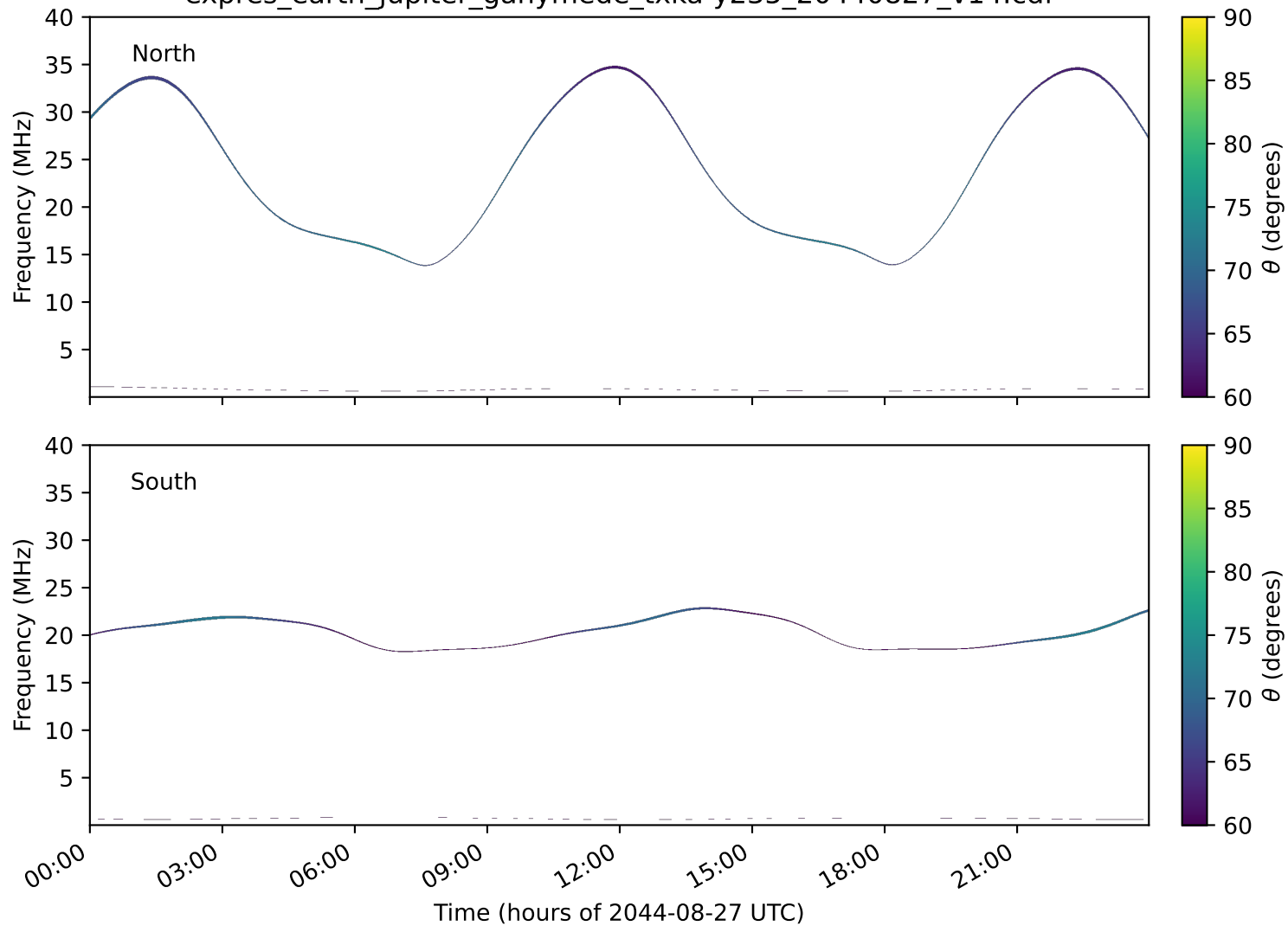
expres_earth_jupiter_ganymede_txka-y235_20440827_v14.cdf
