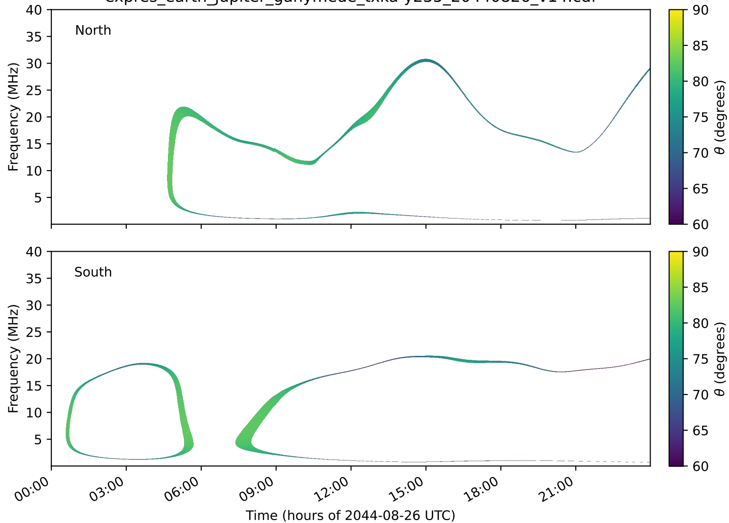
expres_earth_jupiter_ganymede_txka-y235_20440826_v14.cdf
