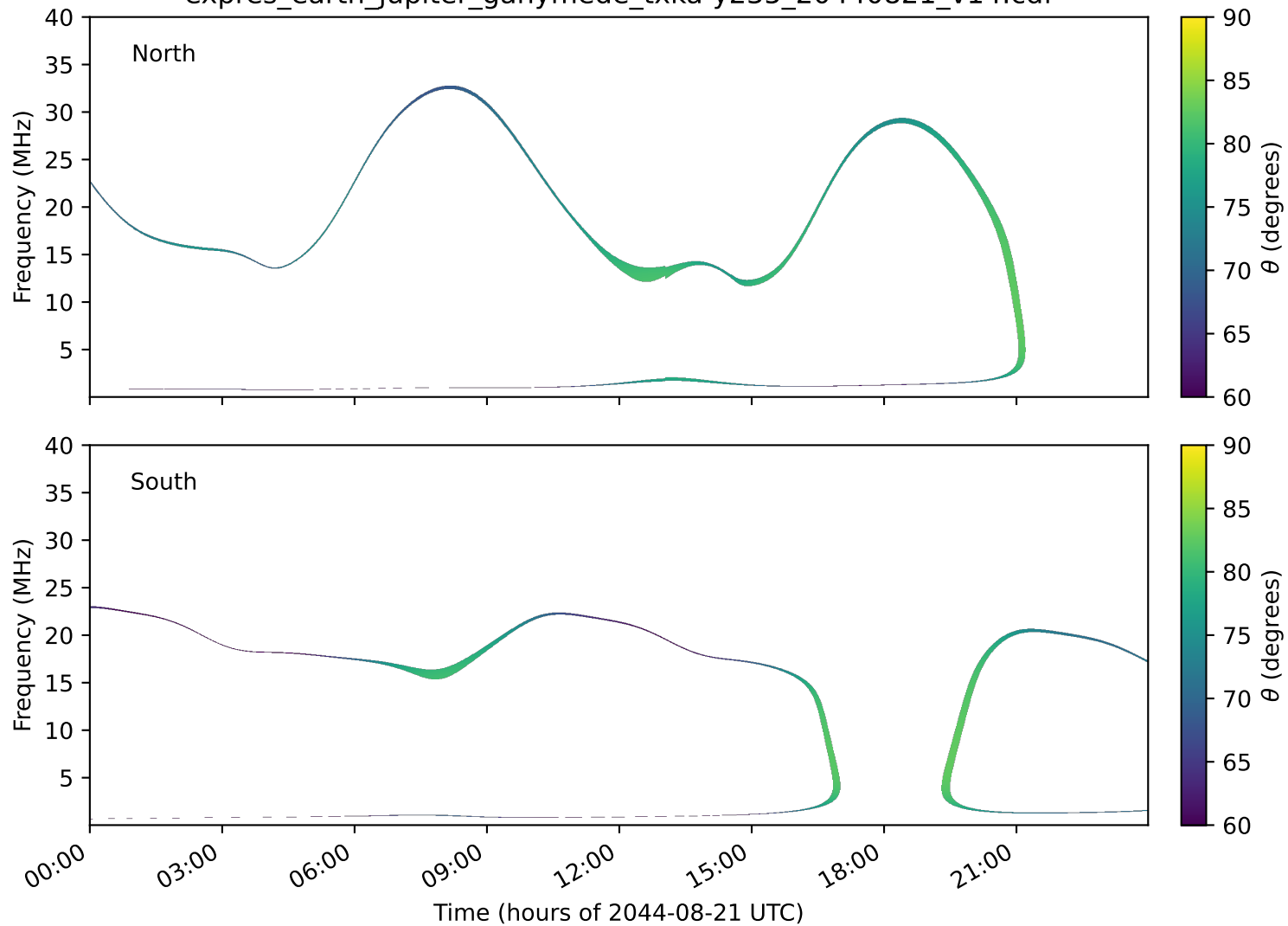
expres_earth_jupiter_ganymede_txka-y235_20440821_v14.cdf
