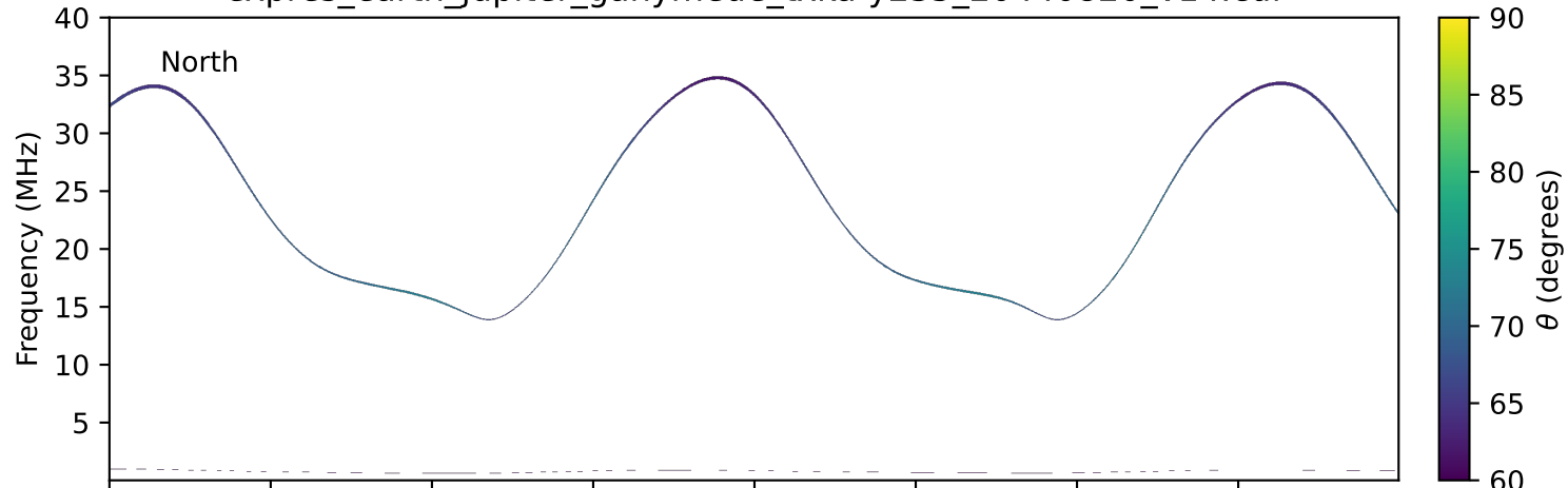
expres_earth_jupiter_ganymede_txka-y235_20440820_v14.cdf
