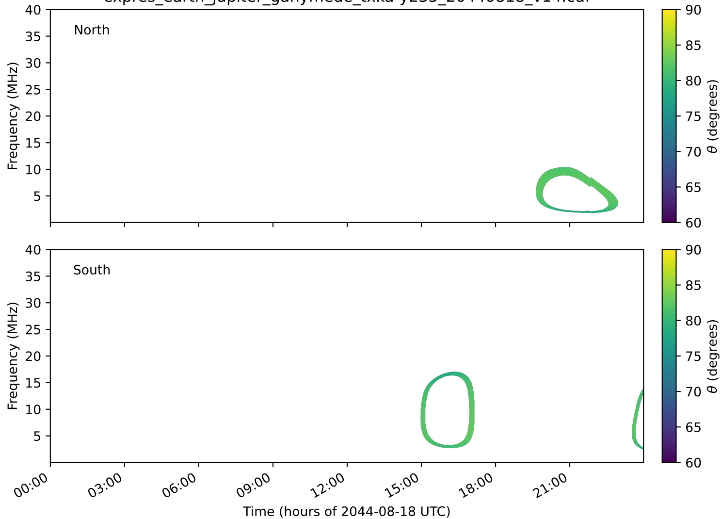
expres_earth_jupiter_ganymede_txka-y235_20440818_v14.cdf
