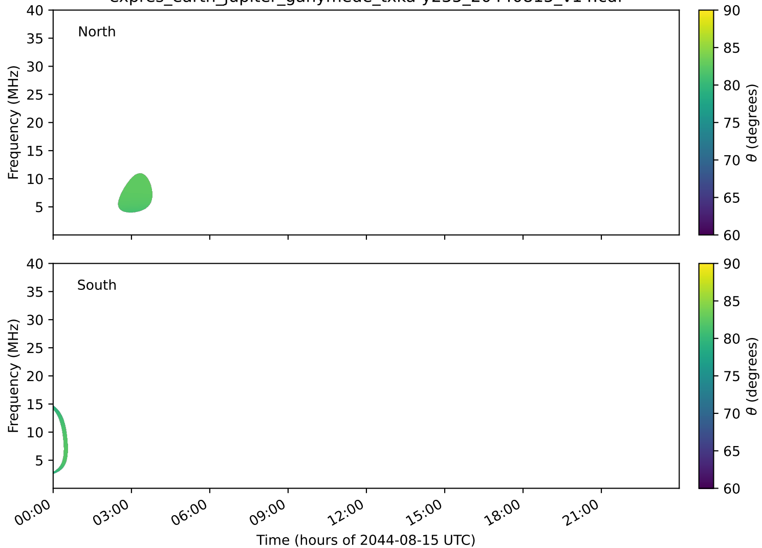
expres_earth_jupiter_ganymede_txka-y235_20440815_v14.cdf
