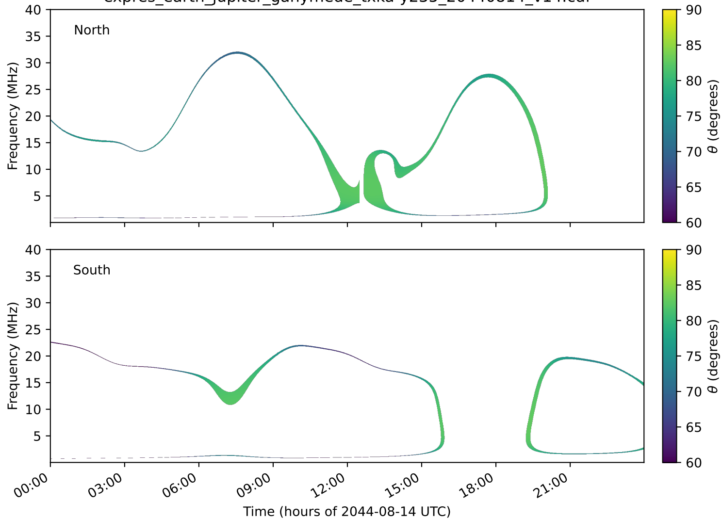
expres_earth_jupiter_ganymede_txka-y235_20440814_v14.cdf
