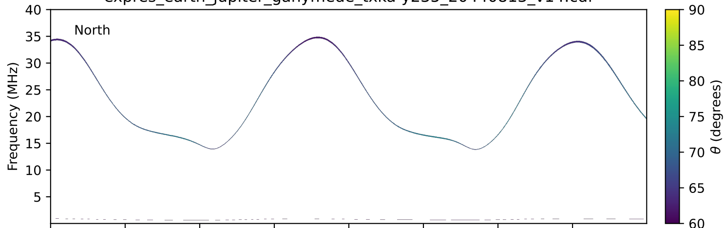
expres_earth_jupiter_ganymede_txka-y235_20440813_v14.cdf
