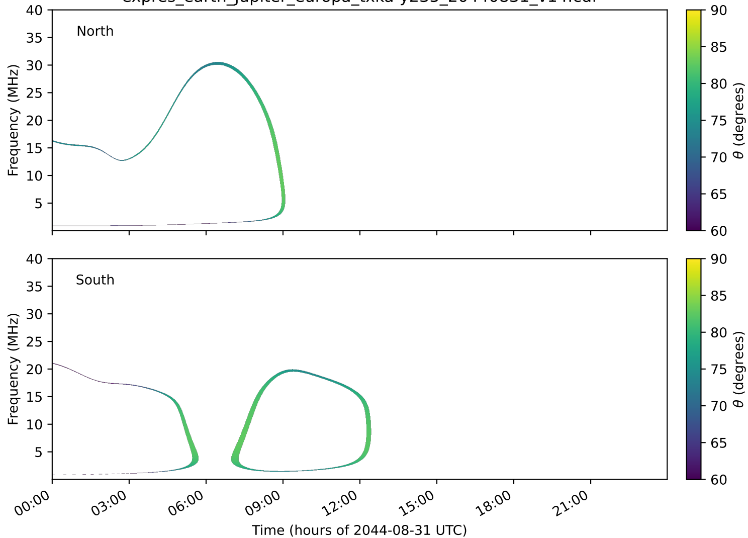
expres_earth_jupiter_europa_txka-y235_20440831_v14.cdf
