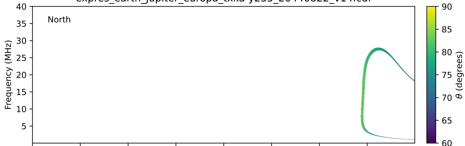
expres_earth_jupiter_europa_txka-y235_20440822_v14.cdf
