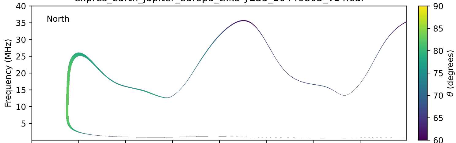
expres_earth_jupiter_europa_txka-y235_20440805_v14.cdf
