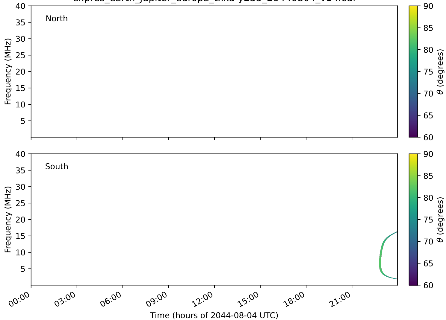
expres_earth_jupiter_europa_txka-y235_20440804_v14.cdf
