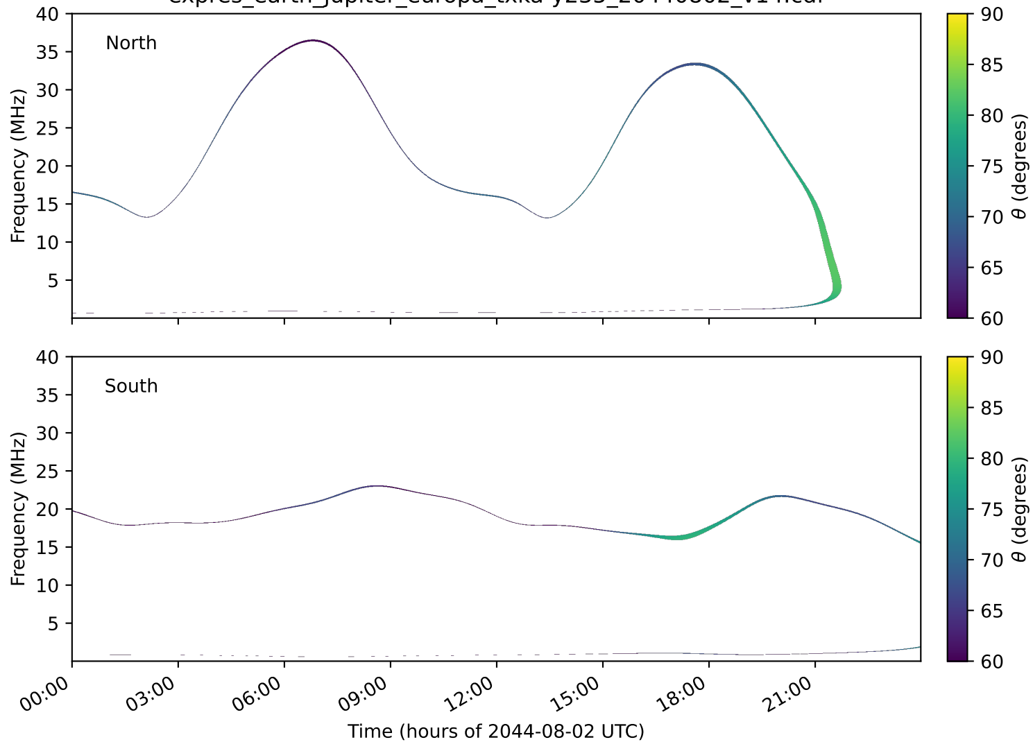
expres_earth_jupiter_europa_txka-y235_20440802_v14.cdf
