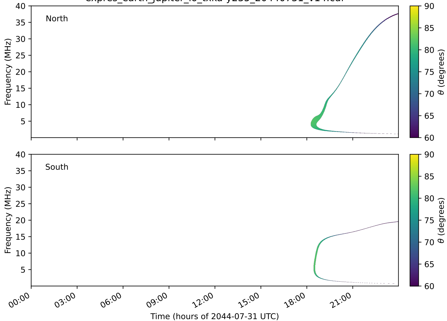
expres_earth_jupiter_io_txka-y235_20440731_v14.cdf
