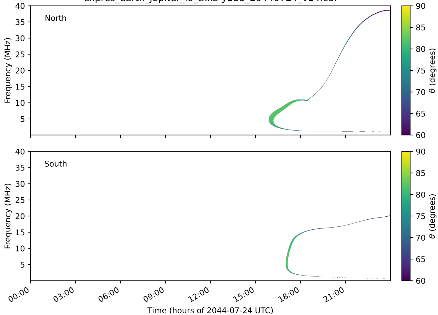
expres_earth_jupiter_io_txka-y235_20440724_v14.cdf
