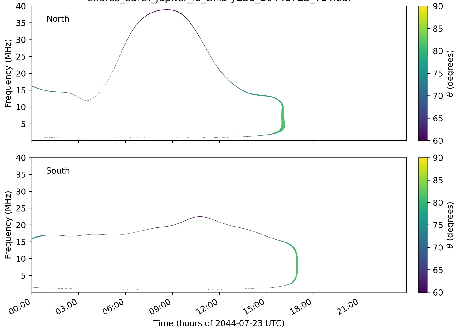
expres_earth_jupiter_io_txka-y235_20440723_v14.cdf
