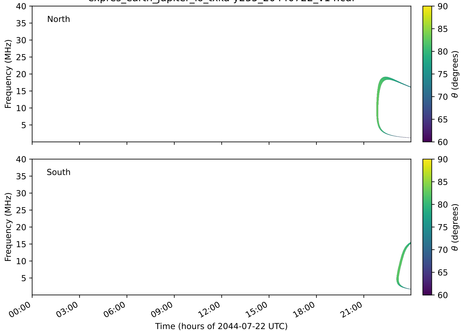
expres_earth_jupiter_io_txka-y235_20440722_v14.cdf
