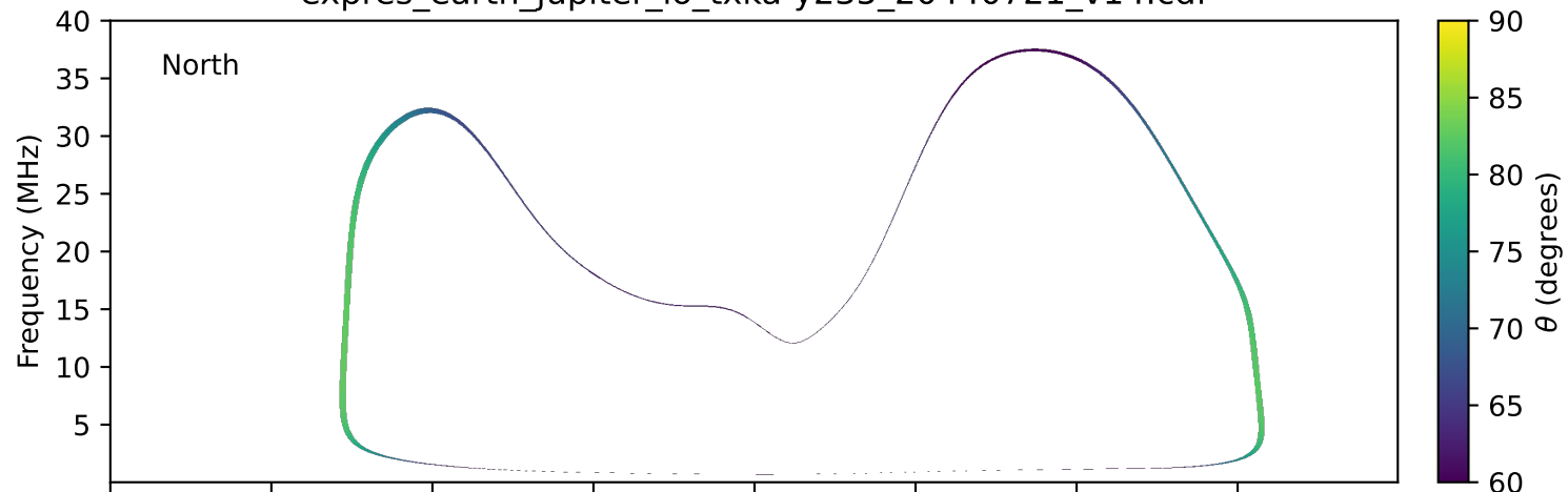
expres_earth_jupiter_io_txka-y235_20440721_v14.cdf
