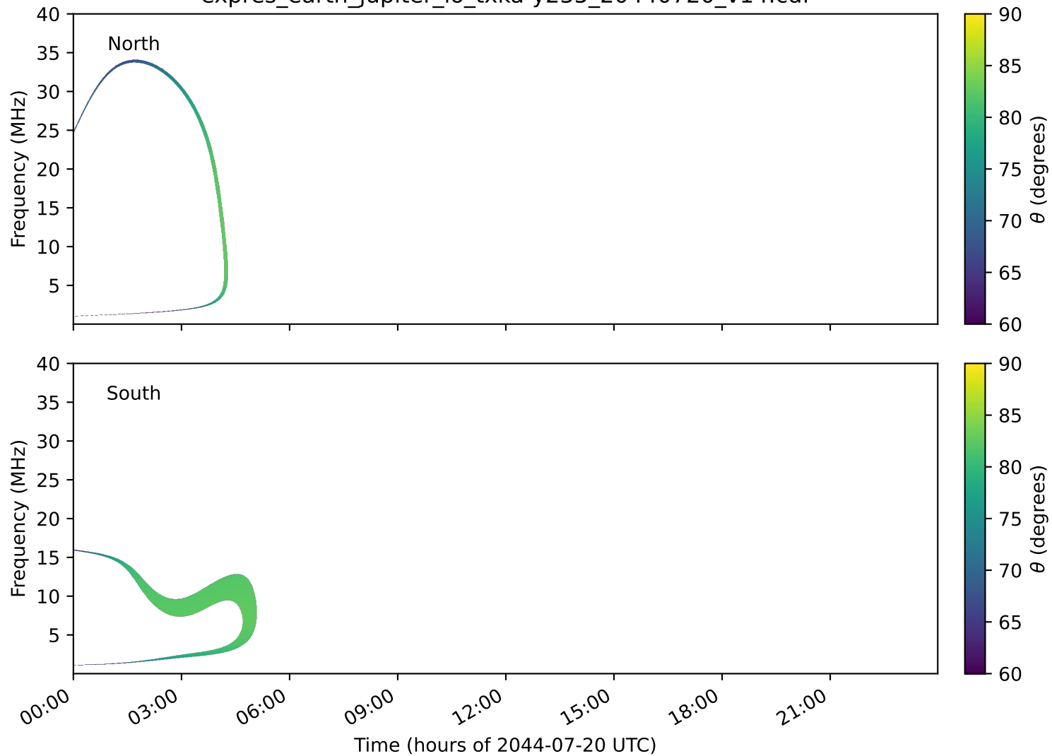
expres_earth_jupiter_io_txka-y235_20440720_v14.cdf
