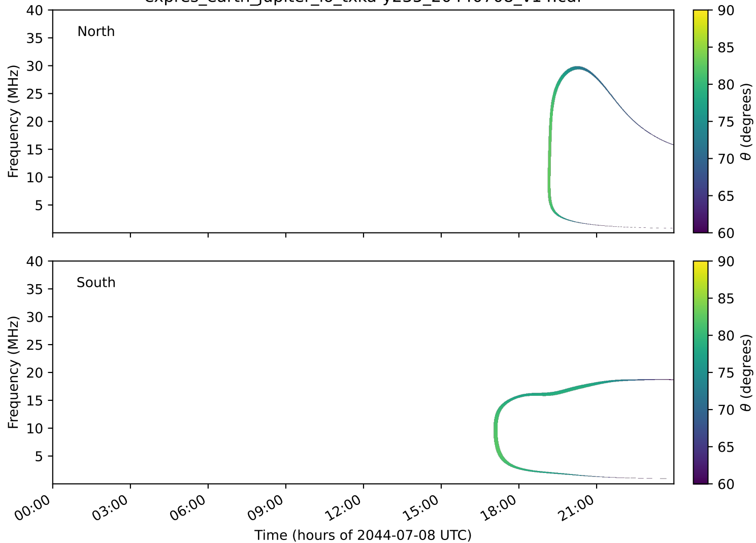
expres_earth_jupiter_io_txka-y235_20440708_v14.cdf
