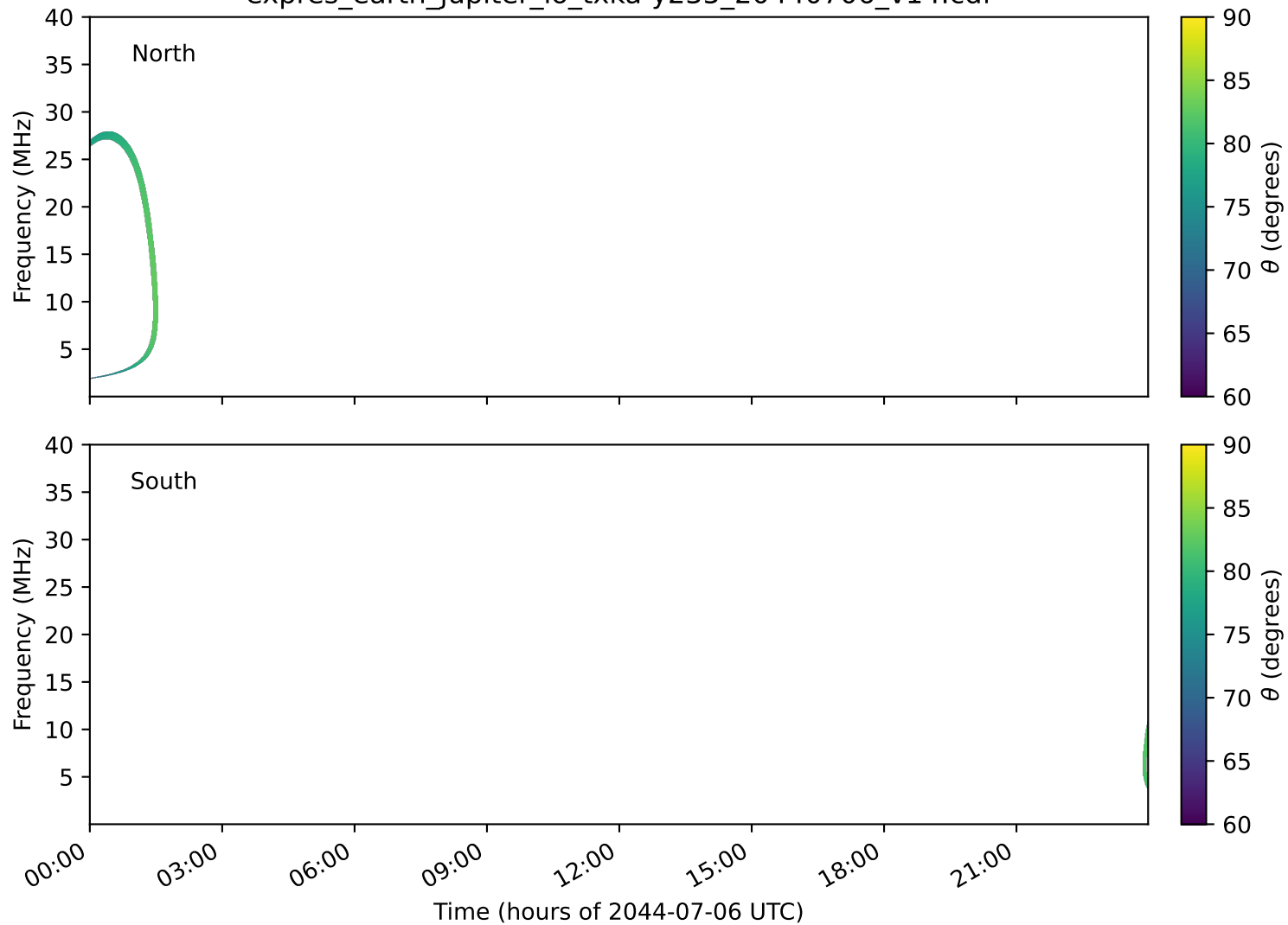
expres_earth_jupiter_io_txka-y235_20440706_v14.cdf
