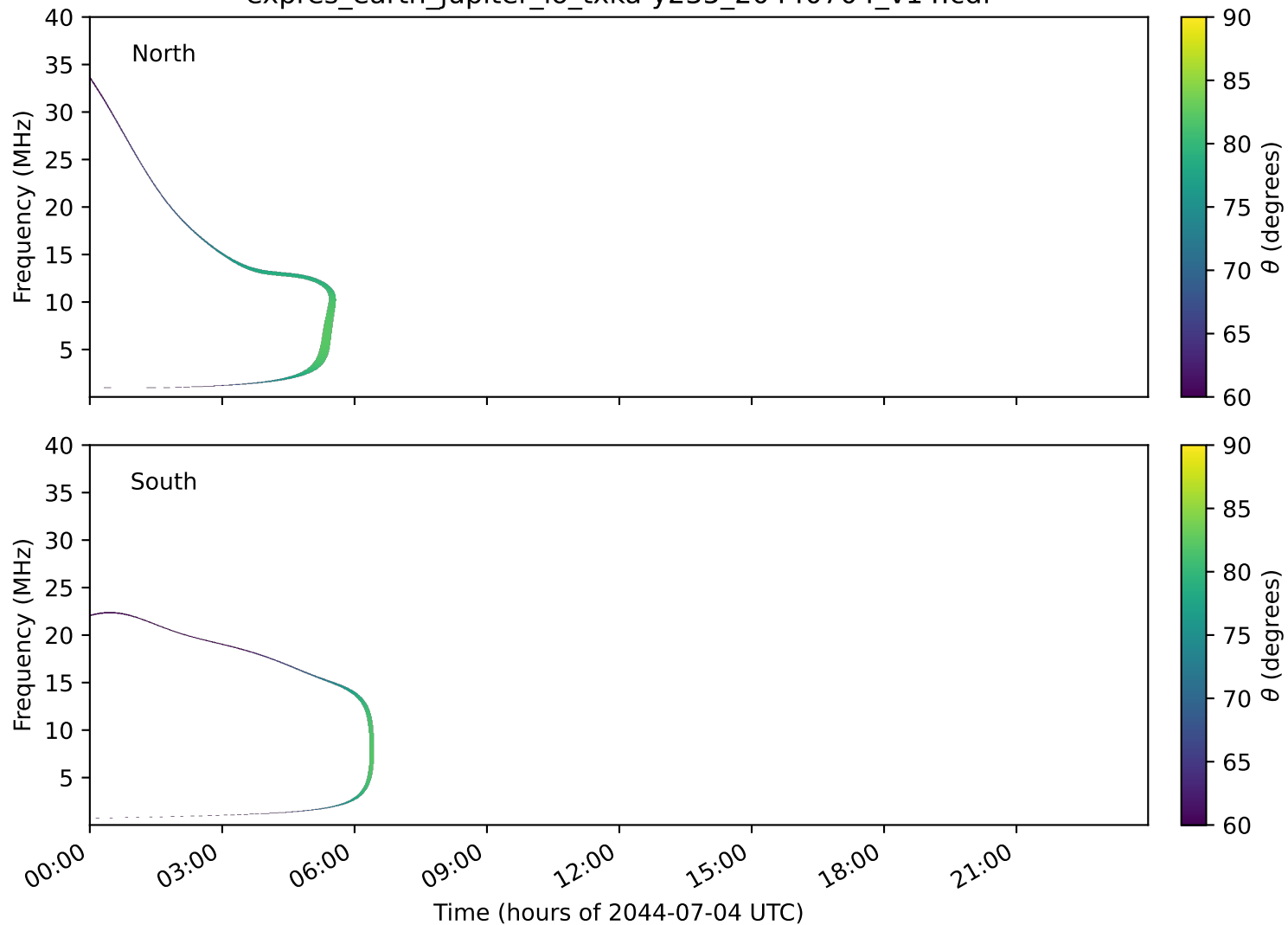
expres_earth_jupiter_io_txka-y235_20440704_v14.cdf
